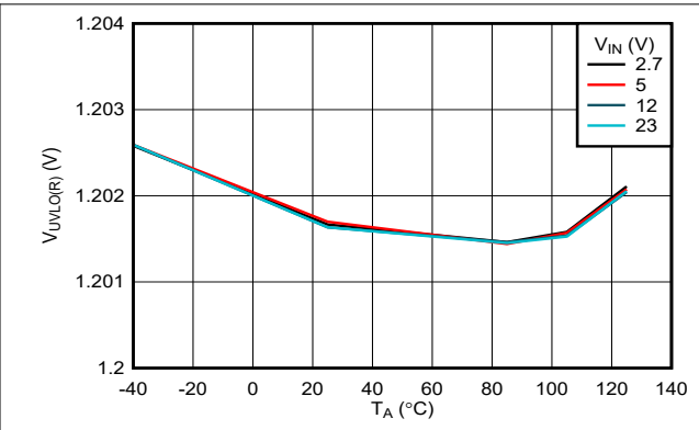
图 7-9. EN/UVLO Rising Threshold vs Temperature
