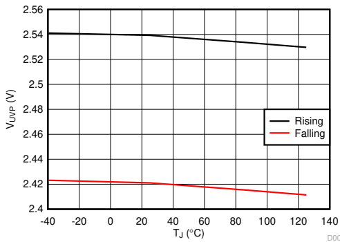
图 7-1. Supply UVP Threshold vs Temperature
