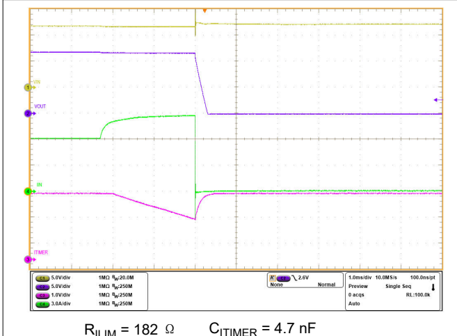
图 7-28. Circuit Breaker With Transient Overcurrent Blanking
