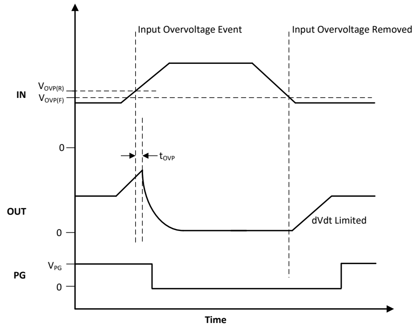
图 8-2. Overtolerance Response
