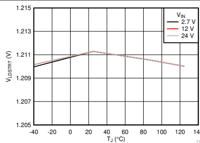
图 7-16. LDSTRT Threshold Voltage vs Temperature
