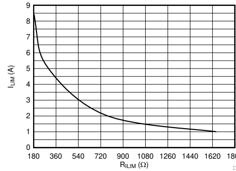
图 7-10. Output Current Limit ( I_{LIM} ) vs R_{LIM}
