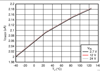
图 7-14. ITIMER Discharge Current vs Temperature
