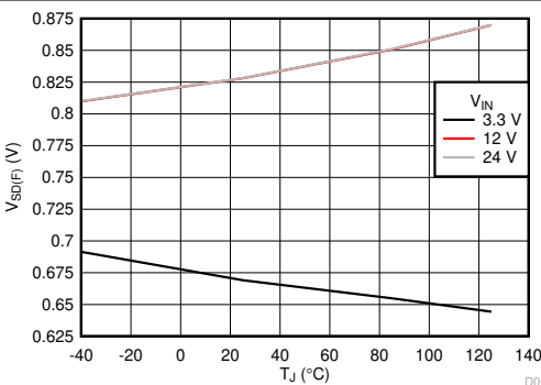
图 7-7. EN/UVLO Falling Threshold for Lowest Current Consumption
