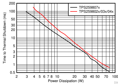
图 7-23. Thermal Shutdown Plot - Inrush/Overload
