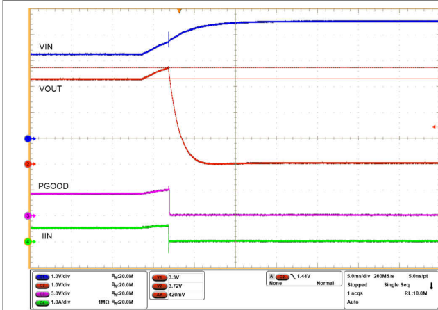
图 9-19. Overvoltage Cut-off at 3.7 V with TPS259802O Device
