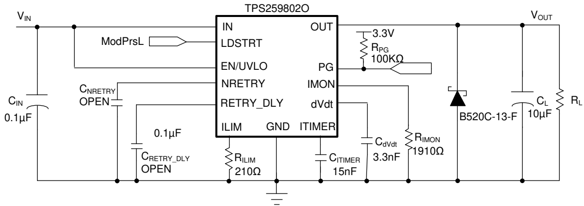
图 9-14. TPS2598020 Configured for a 3.3-V Power Rail Path Protection in Optical Module
