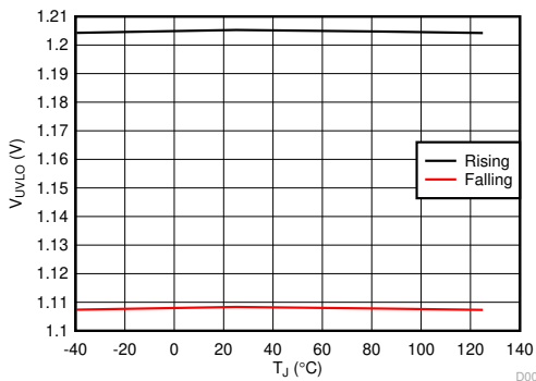
图 7-5. EN/UVLO Threshold vs Temperature
