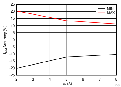
图 7-11. Output Current Limit ( I_{LIM} ) Accuracy
