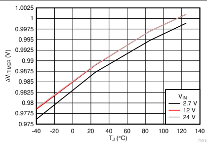
图 7-13. ITIMER Voltage Threshold Delta vs Temperature
