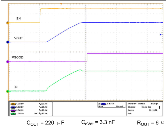
图 7-26. Startup With EN Into Resistive Load - dVdt Limited
