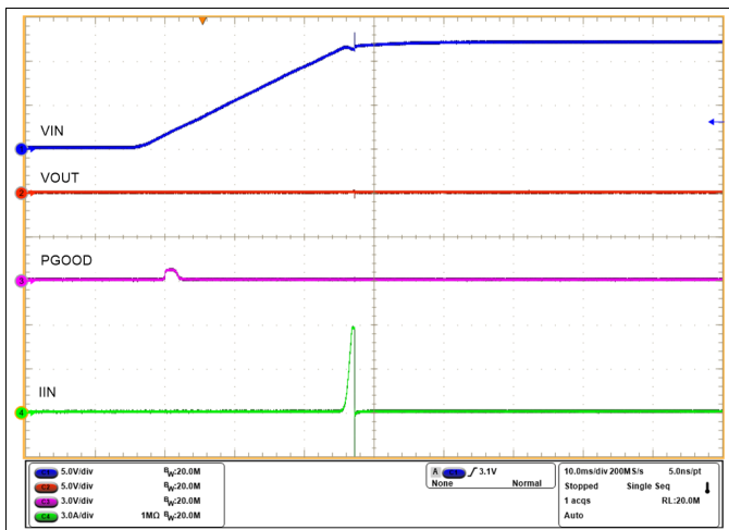
图 60. Power-Up With Short-Circuit on Output
