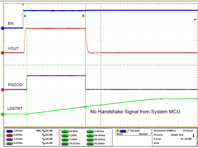
图 63. Unsuccessful Load Handshake (LDSTRT)
