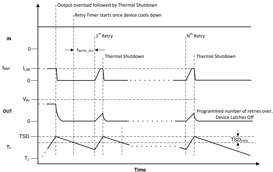
图 51. Auto-Retry After Fault
