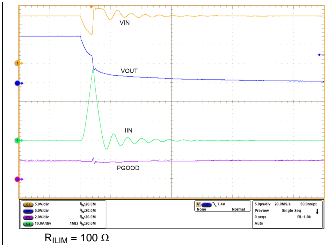
图 39. Output Hard Short-Circuit While ON (Zoomed In)
