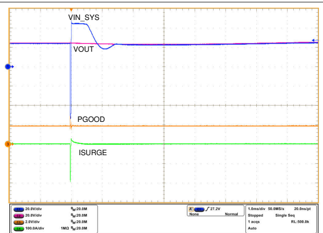
图 10-10. -500-V, 2-Ω Surge Response
