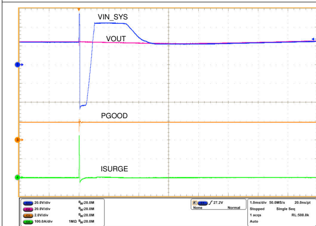
图 10-9. 500-V, 2-Ω Surge Response
