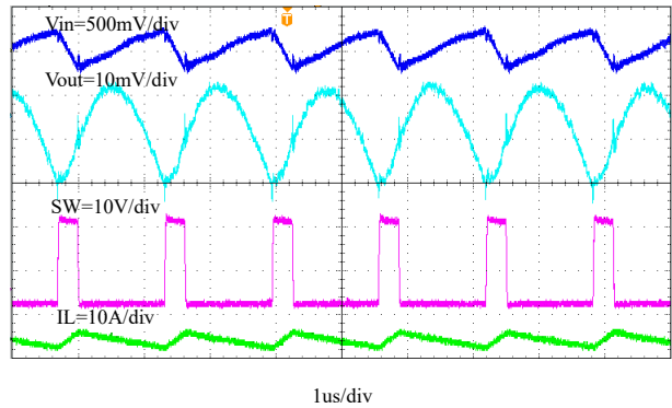
1us/div Figure 8-9. Output Voltage Ripple, Iout = 8 A
