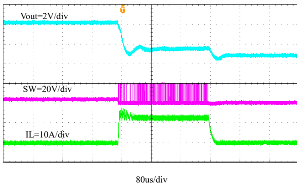
80us/div Figure 8-12. Normal Operation to Output Hard Short
