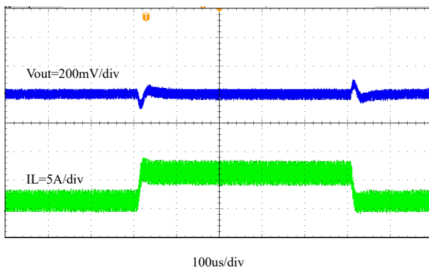
100us/div Figure 8-10. Transient Response, 1.6 A to 6.4 A with 2.5 A/us SR
