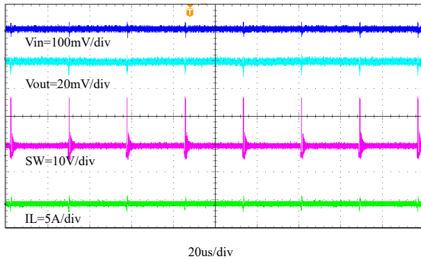
20us/div Figure 8-8. OOA Mode Output Voltage Ripple, Iout = 0 A
