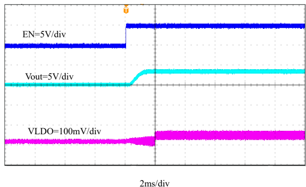
2ms/div Figure 8-13. LDO Switch Over
