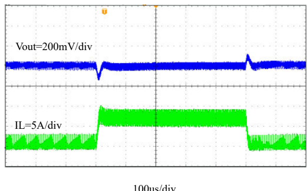
100us/div Figure 8-11. Transient Response, 0.8 A to 7.2 A with 2.5 A/us SR
