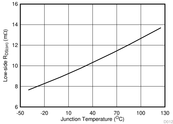
Figure 6-7. Low-Side R_{DS(on)} vs Junction Temperature
