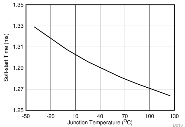
Figure 6-12. Soft-Start Time vs Junction Temperature
