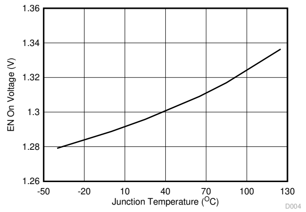
Figure 6-4. Enable On Voltage vs Junction Temperature
