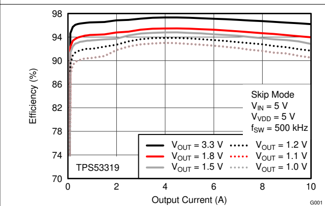
图 7-21. Efficiency vs Output Current
