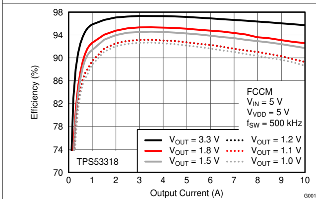
图 7-26. Efficiency vs Output Current
