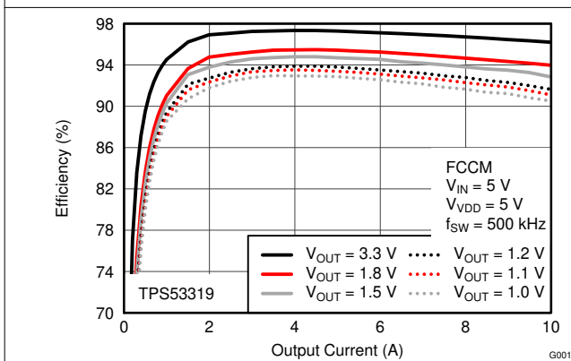
图 7-20. Efficiency vs Output Current
