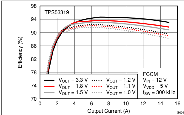
图 7-18. Efficiency vs Output Current
