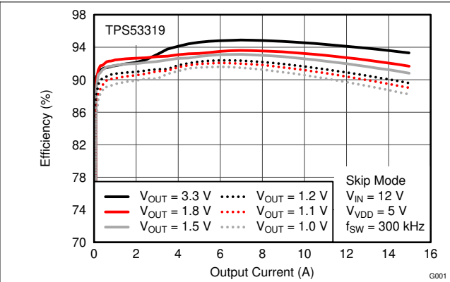
图 7-19. Efficiency vs Output Current
