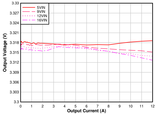
图 6-7. Output Voltage Regulation vs Output Current, V_{OUT} = 3.3\text{ V} , F_{SW} = 1\text{ MHz}
