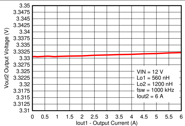
图 8-8. V_{OUT2} Cross Regulation
