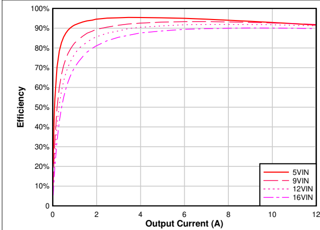
图 6-3. Efficiency vs Output Current, V_{OUT} = 3.3\text{ V} , F_{SW} = 1\text{ MHz}
