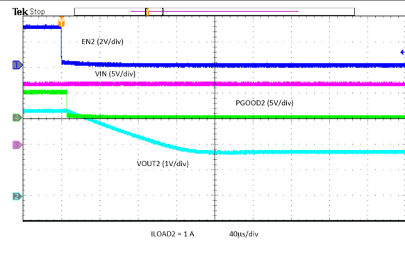
图 8-22. Power Down with EN 2 with Pre Bias
