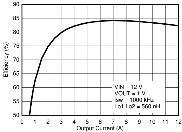
图 8-34. Efficiency
