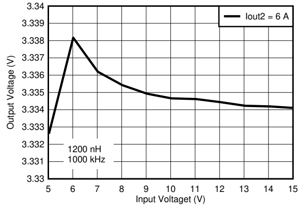
图 8-10. Line Regulation V_{OUT2}
