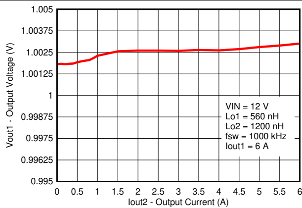
图 8-7. V_{OUT1} Cross Regulation
