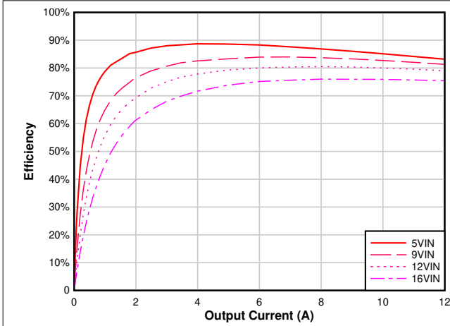
图 6-1. Efficiency vs Output Current, V_{OUT} = 1.0\text{ V} , F_{SW} = 1\text{ MHz}
