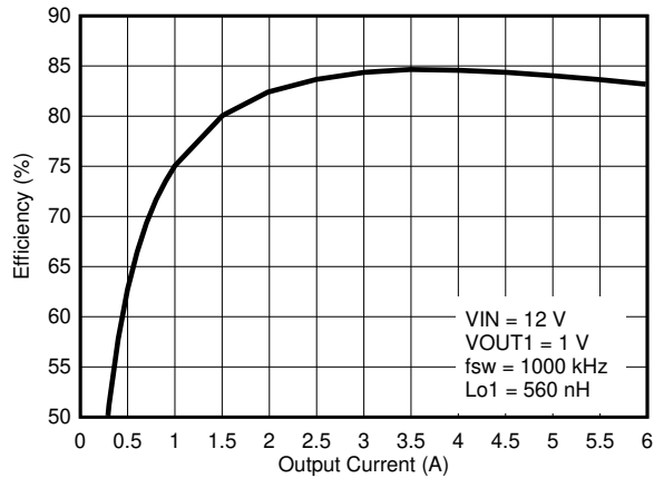
图 8-3. V_{OUT1} Efficiency
