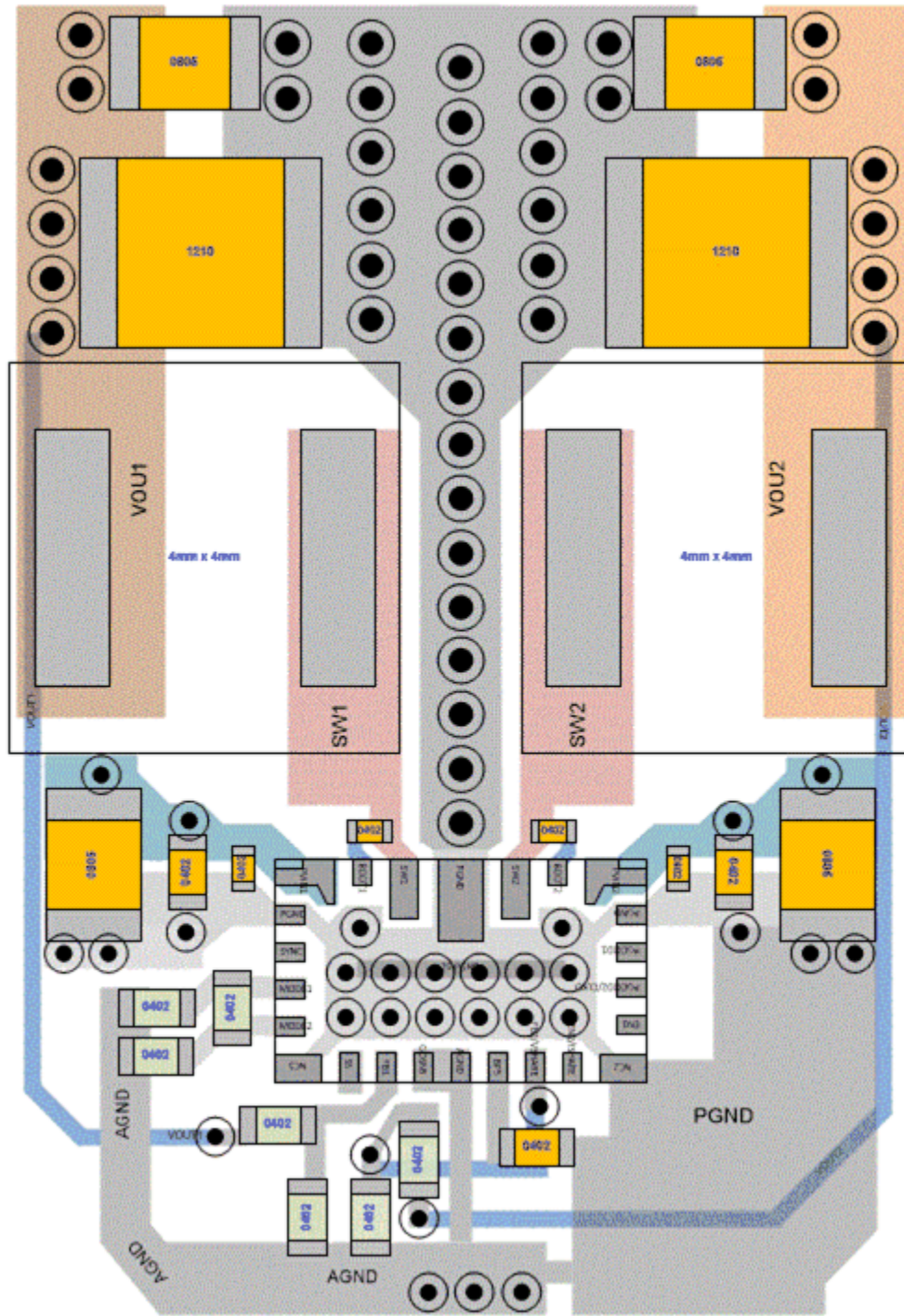
图 10-1. Example PCB Layout for Dual-output Configuration
