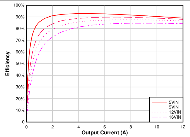
图 6-2. Efficiency vs Output Current, V_{OUT} = 1.8\text{ V} , F_{SW} = 1\text{ MHz}
