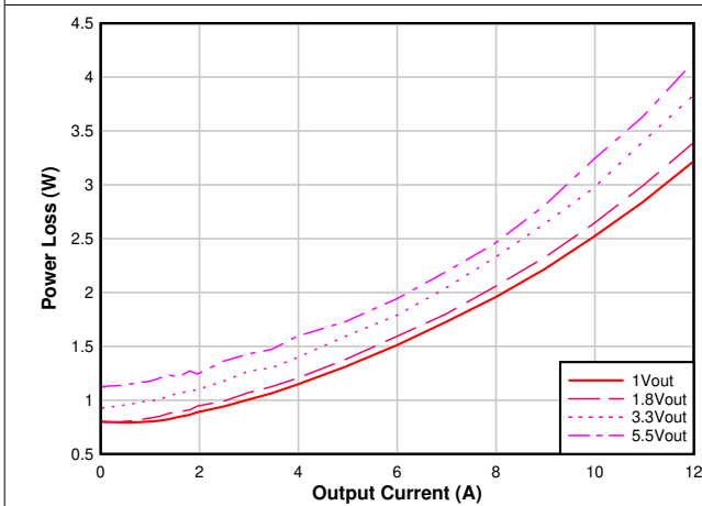
图 6-5. Power Dissipation vs Output Current, V_{IN} = 12\text{ V} , F_{SW} = 1\text{ MHz}
