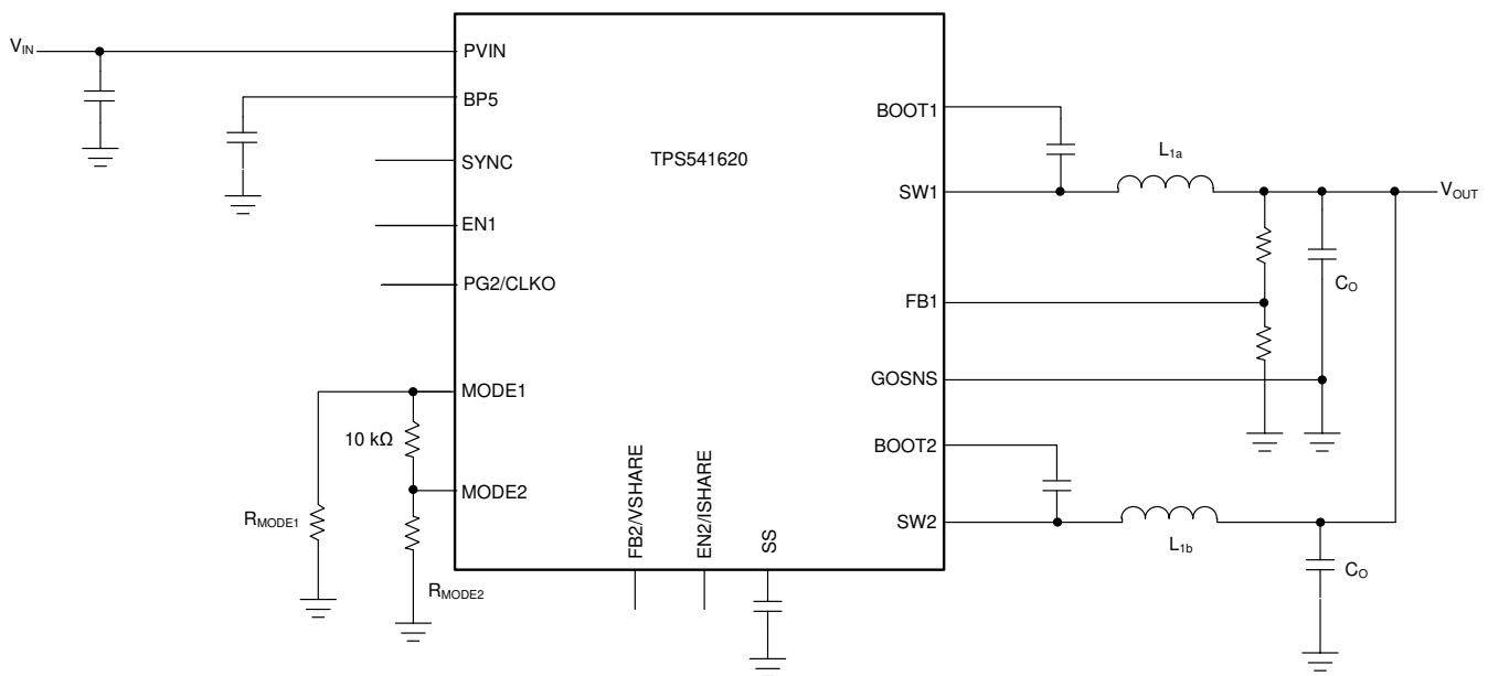
图 7-3. Dual-phase Configuration with External Clock
