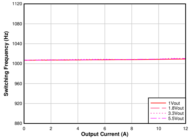
图 6-8. Switching Frequency vs Output Current, V_{IN} = 12\text{ V} , F_{SW} = 1\text{ MHz}
