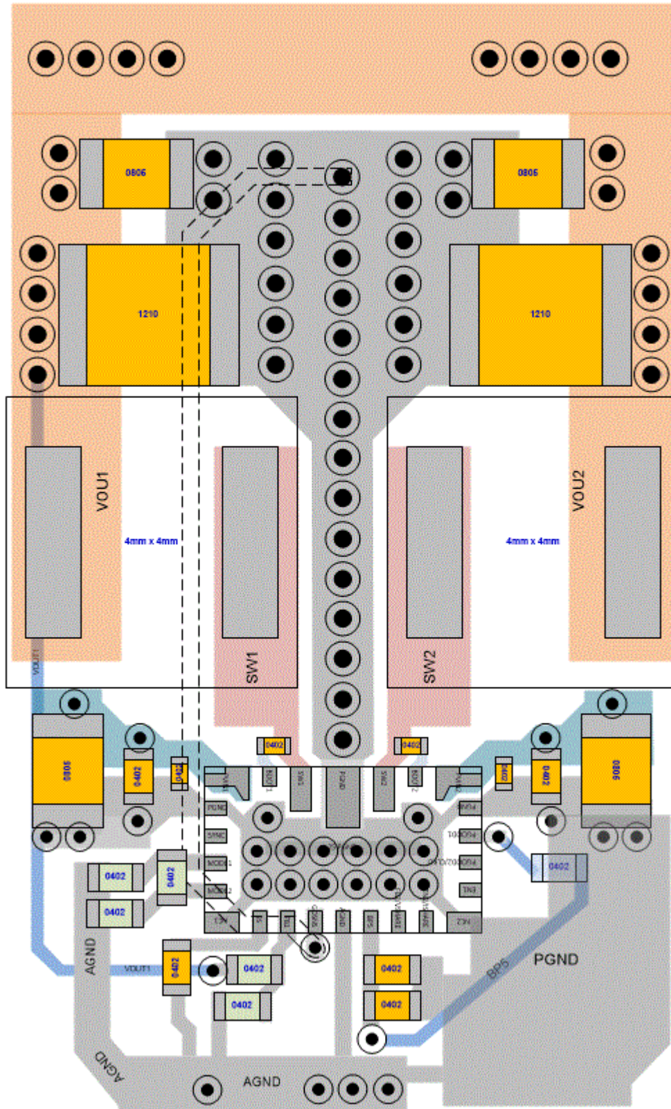
图 10-2. Example PCB Layout for Dual-phase Configuration
