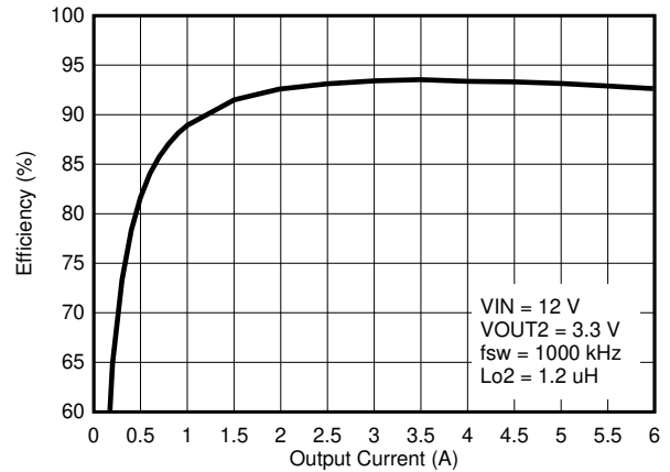
图 8-4. V_{OUT2} Efficiency
