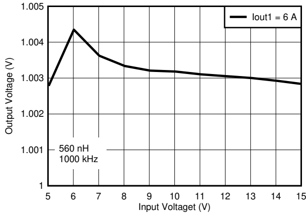
图 8-9. Line Regulation V_{OUT1}
