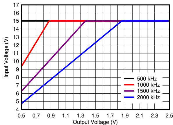
图 8-33. Maximum Input Voltage Versus Output Voltage
