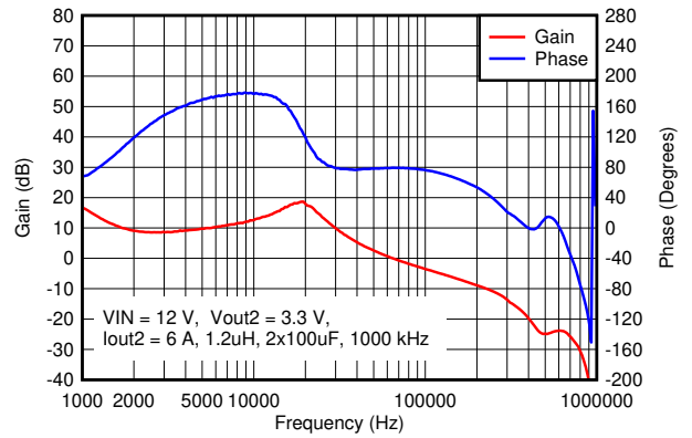
图 8-12. V_{OUT2} Bode Plot
