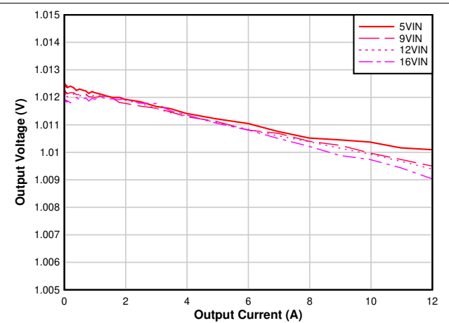
图 6-6. Output Voltage Regulation vs Output Current, V_{OUT} = 1.0\text{ V} , F_{SW} = 1\text{ MHz}
