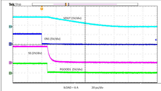
图 8-40. Power Down with EN
