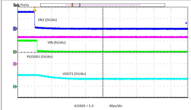
图 8-21. Power Down with EN 1 with Pre Bias
