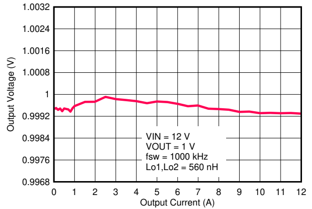
图 8-35. Load Regulation
