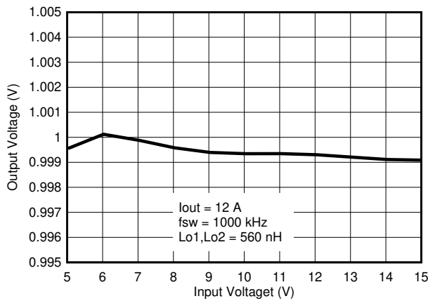
图 8-36. Line Regulation
