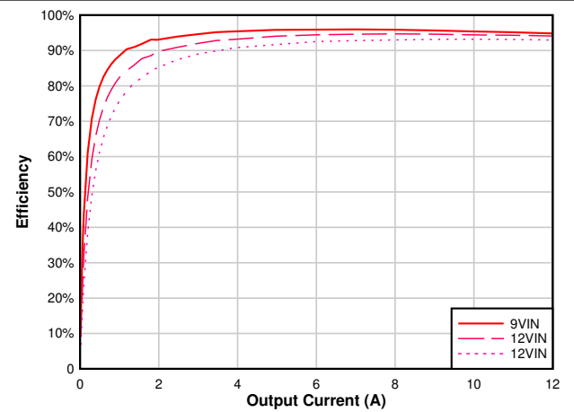
图 6-4. Efficiency vs Output Current, V_{OUT} = 5.5\text{ V} , F_{SW} = 1\text{ MHz}
