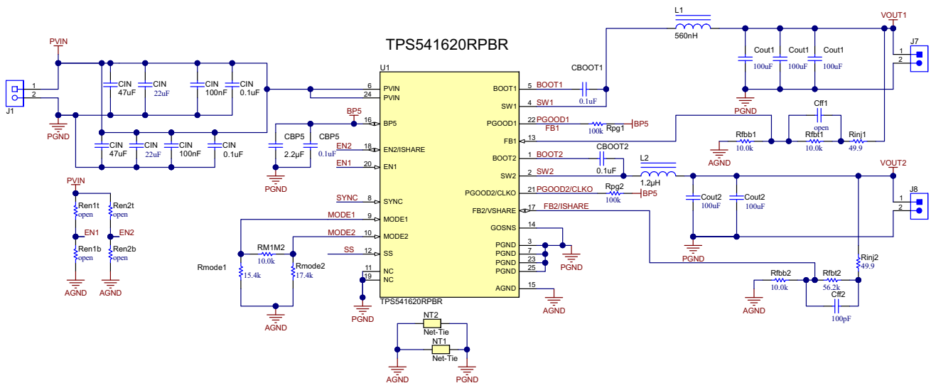
图 8-1. 12-V Input, 1.0-V and 3.3-V Dual Output Regulator Application Schematic
