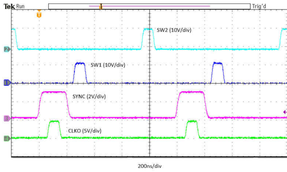
图 8-27. Sync In to SW1 and SW2 Delay
