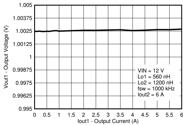
图 8-5. V_{OUT1} Load Regulation
