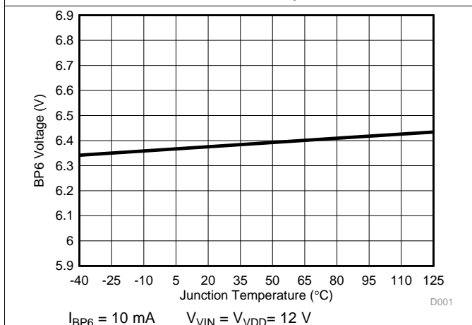
Figure 9. BP6 Voltage vs. Junction Temperature
