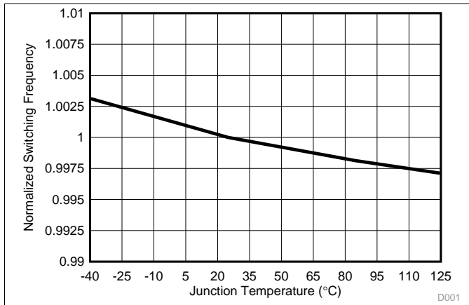
Figure 7. Normalized Switching Frequency vs. Junction Temperature
