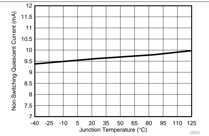
Figure 8. Non-Switching Input Current ( I_{VDD} ) vs. Junction Temperature
