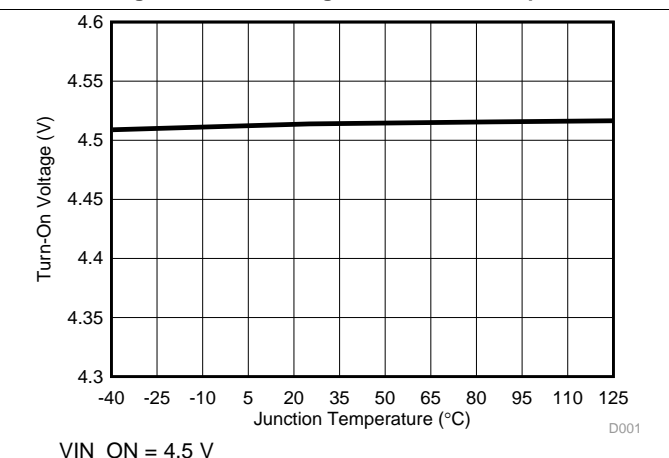
Figure 12. Turn-On Voltage vs. Junction Temperature
