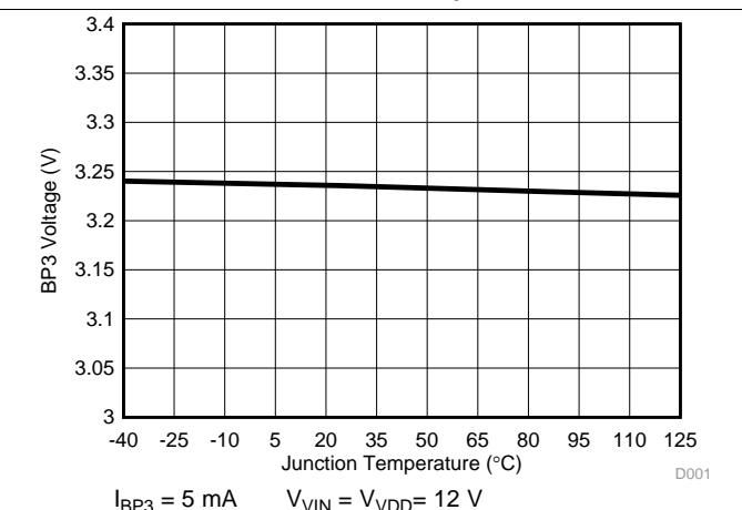
Figure 10. BP3 Voltage vs. Junction Temperature
