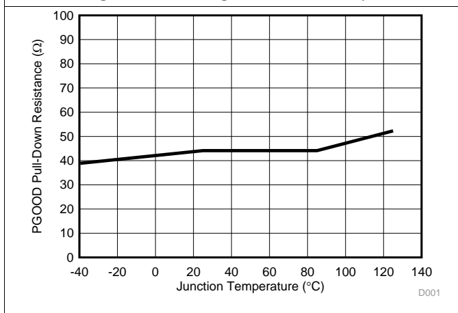
Figure 11. PGOOD Pull-Down Resistance vs. Junction Temperature
