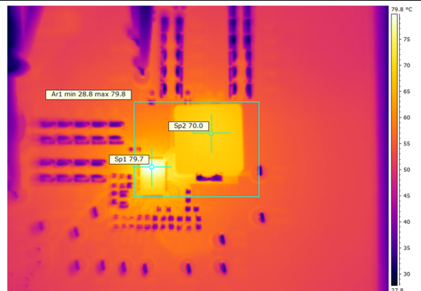
Figure 10. Thermal Image
