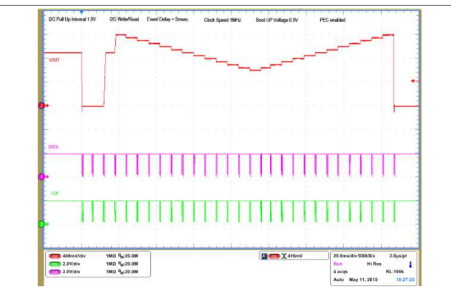
Figure 20. 29 Sequenced Events – I2C Write
