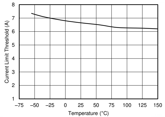
图 7-2. Switch Current Limit vs Temperature
