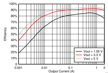
TPS562202S Efficiency
