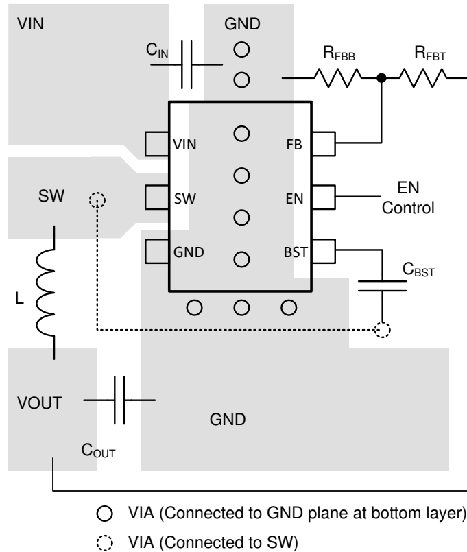
Figure 11-1. TPS562202S Layout
