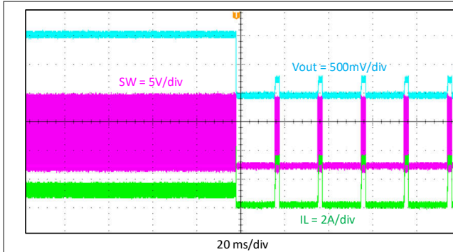
Figure 9-14. OC
