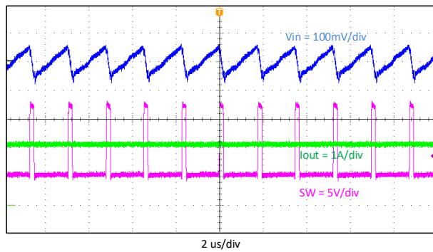
Figure 9-4. Input Voltage Ripple I_{out} = 2\text{ A}
