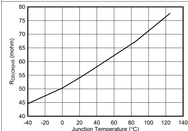
图 6-5. High-Side R_{DS(ON)}
