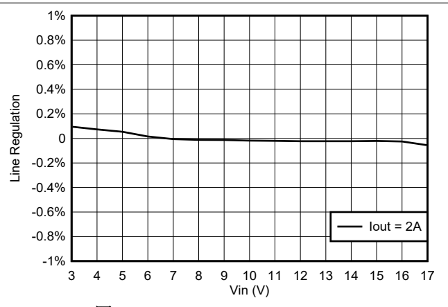
图 8-5. Line Regulation vs V_{IN}
