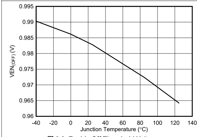
图 6-3. Enable Off Threshold Voltage
