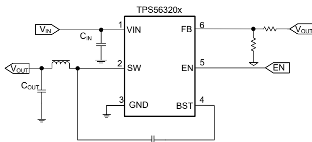
Simplified Schematic
