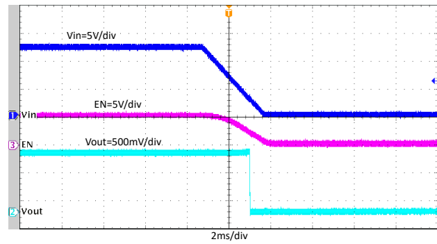
图 8-21. Shutdown with V_{IN} Falling, I_{OUT} = 4 A
