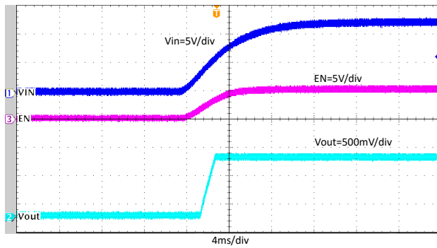
图 8-20. Start-Up with V_{IN} Rising, I_{OUT} = 4 A
