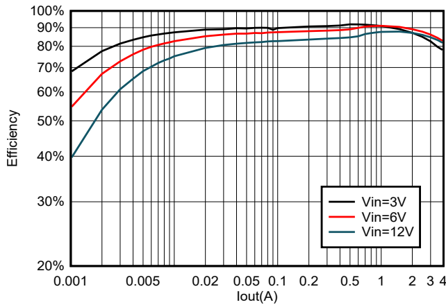
图 6-13. TPS564252 Efficiency at 1.05 V_{OUT} with a 1.5- \mu\text{H} Inductor
