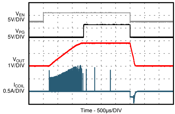
图 9-28. PSM Operation
