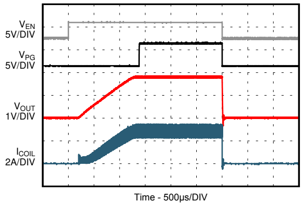
图 9-30. Start-Up with No-Load
