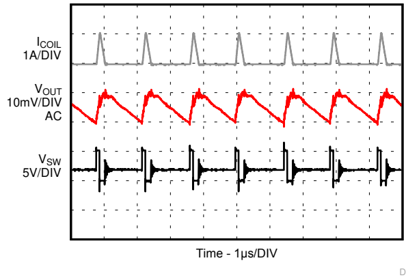
图 9-28. PSM Operation
