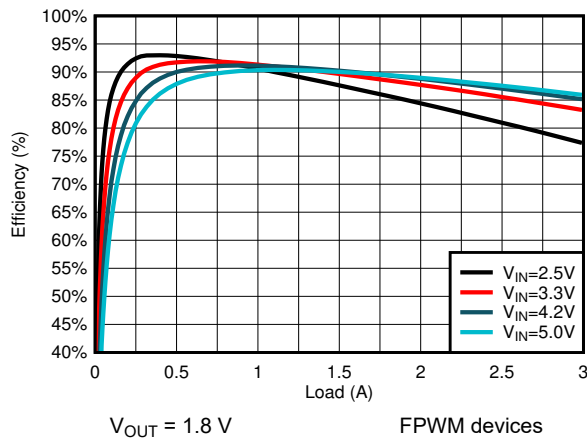
图 9-17. Efficiency
