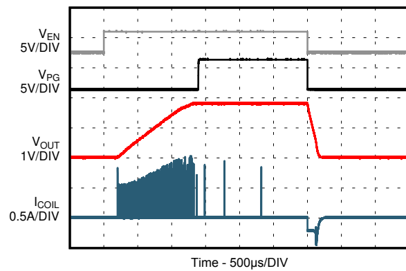
图 9-28. PSM Operation
