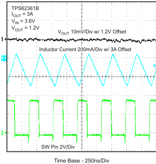
SWITCHING WAVE FORMS I_{OUT} = 3\text{A}
