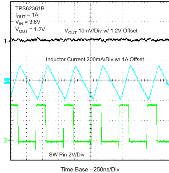
SWITCHING WAVE FORMS I_{OUT} = 1\text{A}
