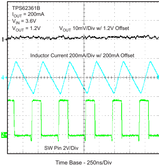
SWITCHING WAVE FORMS I_{OUT} = 200\text{mA}
