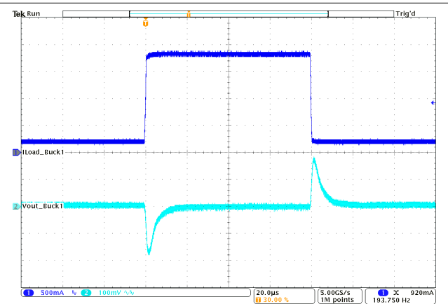
图 10-27. Load Transient Response
