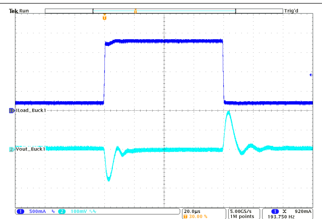
图 10-29. Load Transient Response
