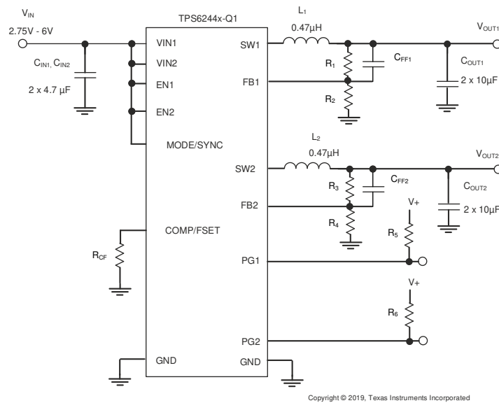
图 8-1. Measurement Setup
