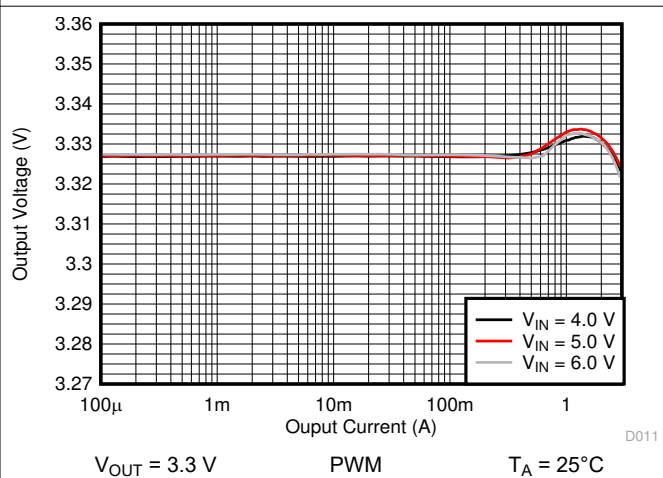
图 10-13. Output Voltage vs Output Current
