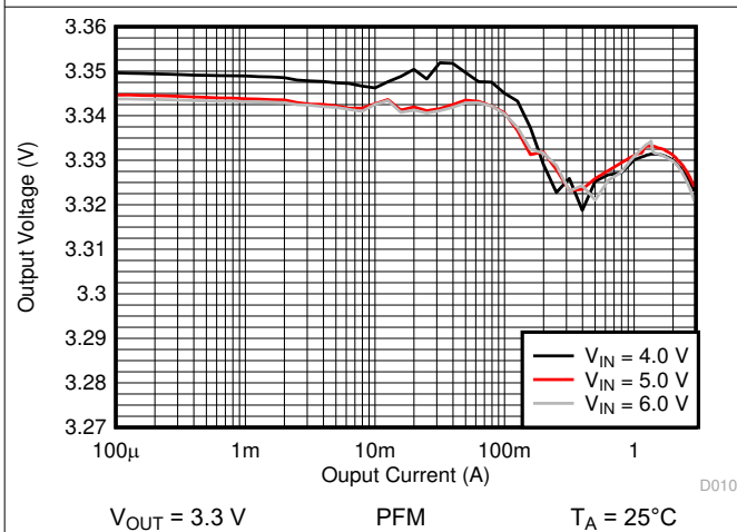
图 10-12. Output Voltage vs Output Current
