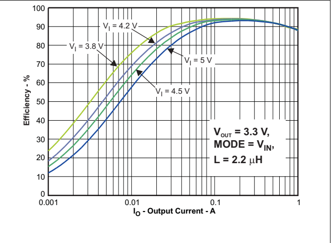
Figure 25. Efficiency vs Output Current for V_{\text{OUT}} = 3.3 \text{ V} (Forced PWM Mode)
