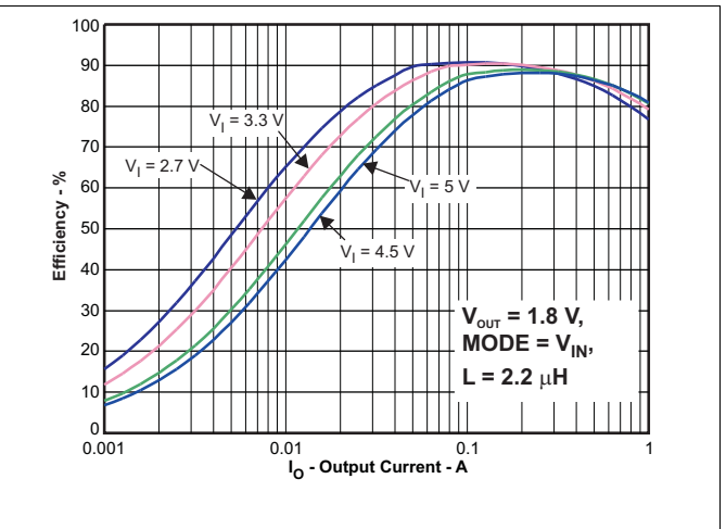
Figure 23. Efficiency vs Output Current for V_{\text{OUT}} = 1.8 \text{ V} (Forced PWM Mode)
