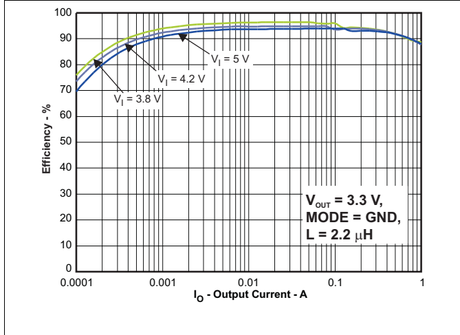
Figure 24. Efficiency vs Output Current for V_{\text{OUT}} = 3.3 \text{ V} (Power-Save Mode)
