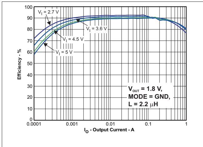
Figure 22. Efficiency vs Output Current for V_{\text{OUT}} = 1.8 \text{ V} (Power-Save Mode)
