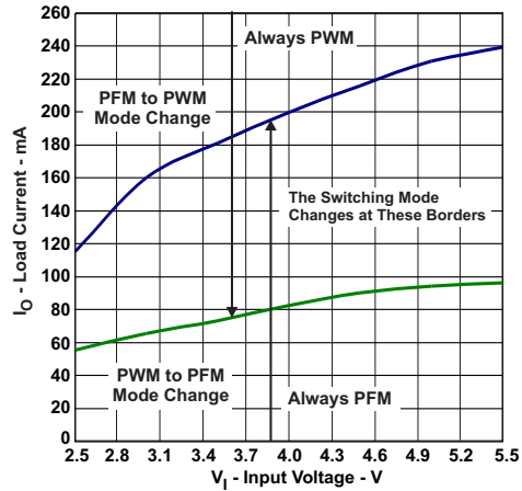
V_{OUT} = 1.2\text{ V} Mode Change
