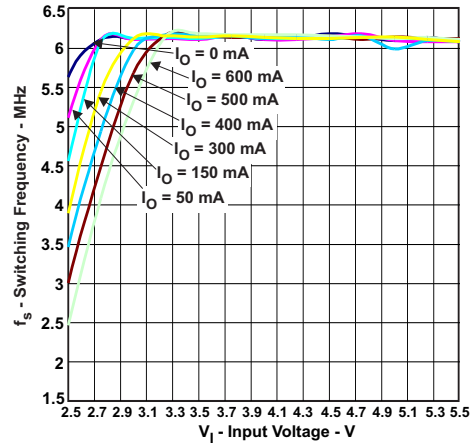
V_{OUT} = 1.82\text{ V}
