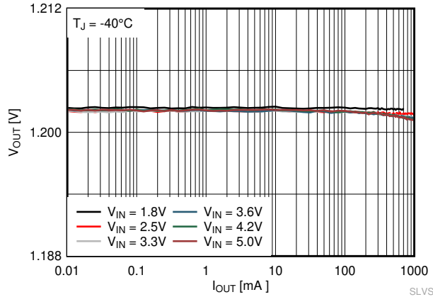
TPS62801 VSEL/MODE = high after start-up V_{OUT} = 1.2\text{ V} Forced PWM mode T_J = -40^\circ\text{C}
