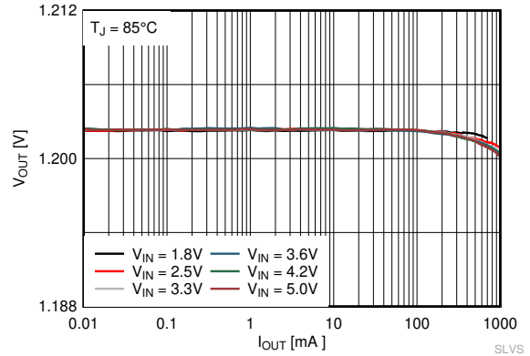
TPS62801 VSEL/MODE = high after start-up V_{OUT} = 1.2\text{ V} Forced PWM mode T_J = 85^\circ\text{C}
