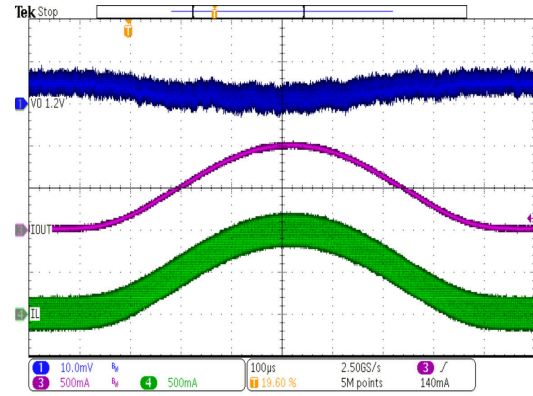
TPS62801 V_{OUT} = 1.2\text{ V} V_{SEL}/MODE = VIN I_{OUT} = 1\text{ mA to }1\text{ A, }1\text{ kHz} (\text{after start-up}) Forced\ PWM\ mode
