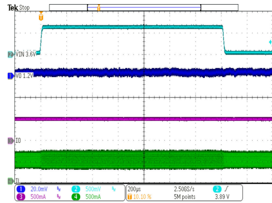
TPS62801 V_{OUT} = 1.2\text{ V} V_{IN} = 3.6\text{ V to }4.2\text{ V} \text{rise / fall time} = 10\ \mu\text{s} I_{OUT} = 500\text{ mA}
