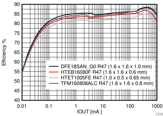
TPS62801 VSEL/MODE = GND, V_{OUT} = 1.2 \text{ V}
