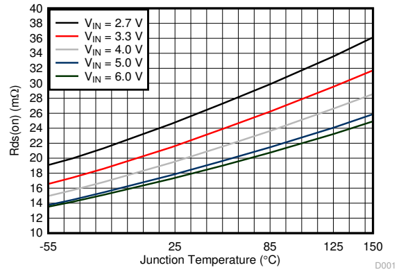
图 7-2. R_{ds(on)} of Low-side Switch
