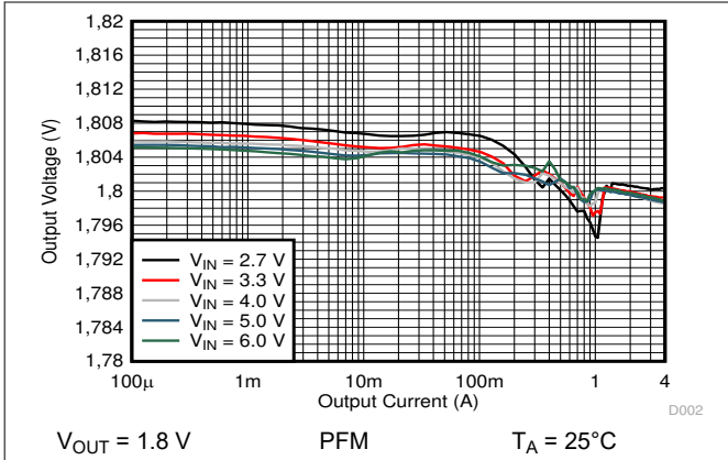
图 10-14. Output Voltage versus Output Current
