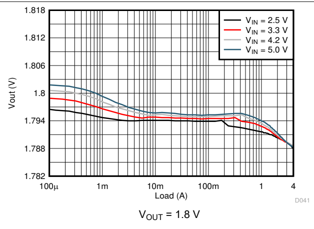
图 9-12. Load Regulation
