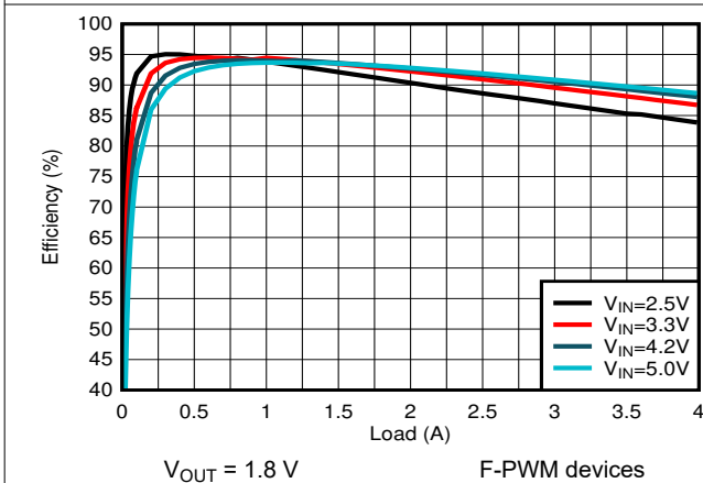
图 9-13. PWM Efficiency
