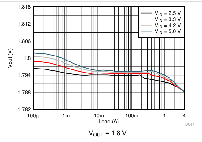
图 9-12. Load Regulation
