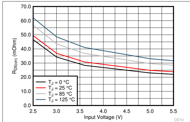
图 7-1. High-Side FET On-Resistance
