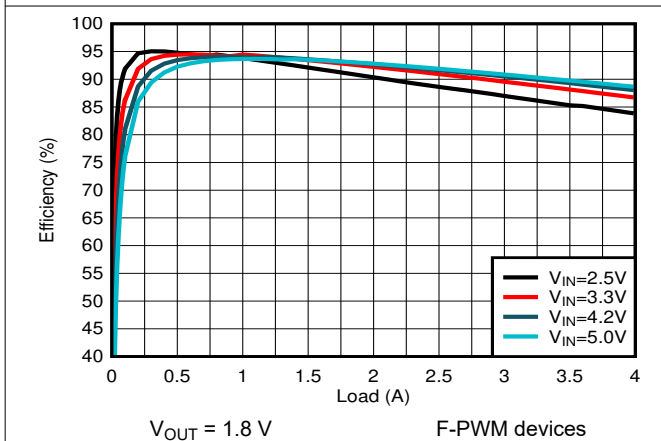
图 9-13. PWM Efficiency
