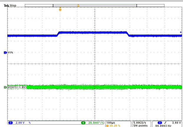
Figure 8-36. Line Transient
