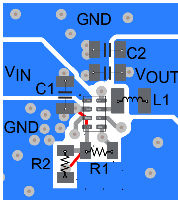
Figure 8-49. PCB Layout Recommendation (RZE Package)
