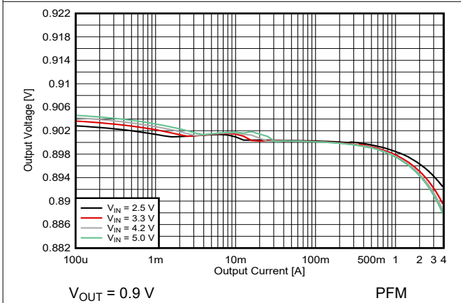
Figure 8-17. Output Voltage versus Output Current
