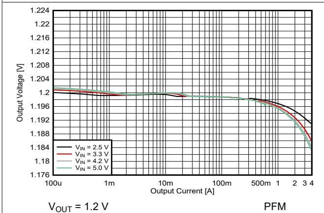
Figure 8-19. Output Voltage versus Output Current
