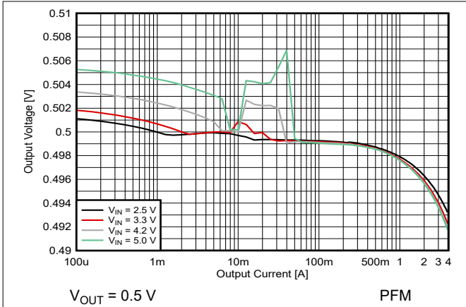
Figure 8-15. Output Voltage versus Output Current
