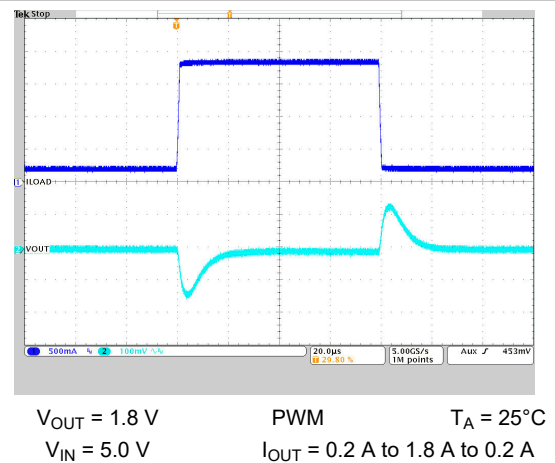
图 10-25. Load Transient Response
