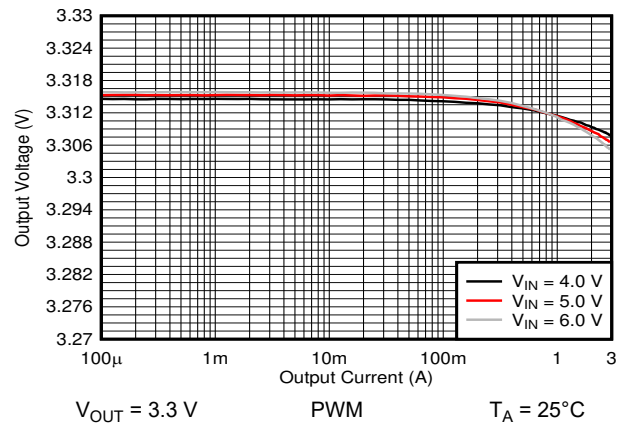
图 10-11. Output Voltage Versus Output Current
