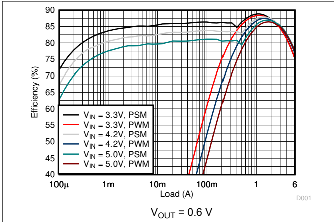
图 9-2. Efficiency
