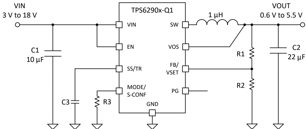
Figure 8-2. Adjustable V O Operation Schematic
