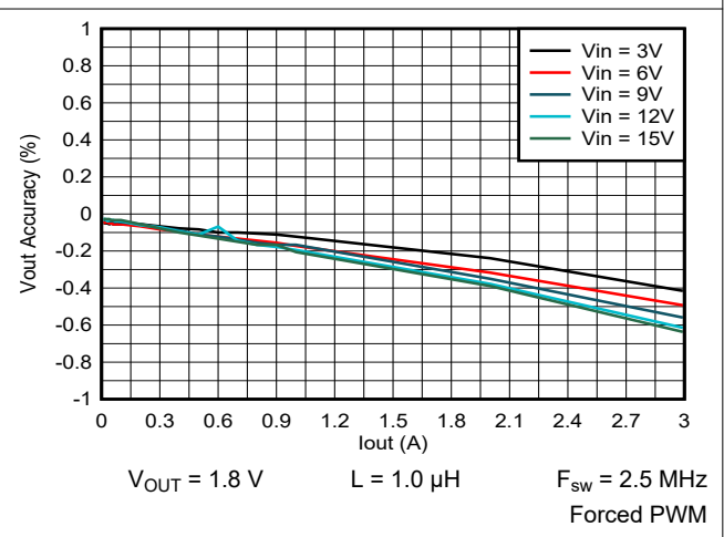
Figure 9-8. Output Voltage vs Output Current
