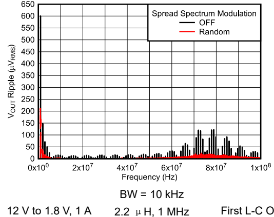
图 6-8. V_{OUT} Ripple FFT After the First L-C Filter
