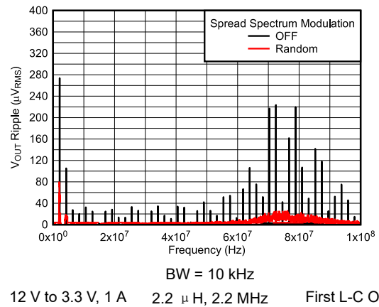
图 6-12. V_{OUT} Ripple FFT After the First L-C Filter
