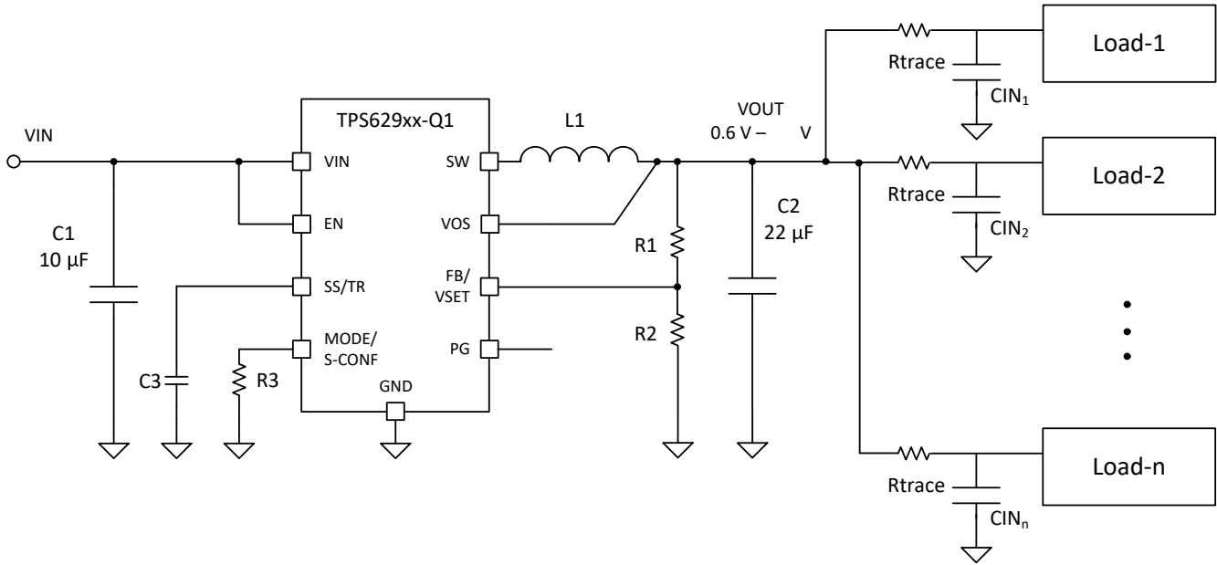
图 9-82. Multiple Loads
