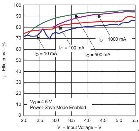
Figure 11. Efficiency vs Input Voltage (TPS63010)
