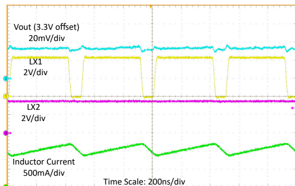
Figure 9-8. Switching Waveforms with 1-A Load
