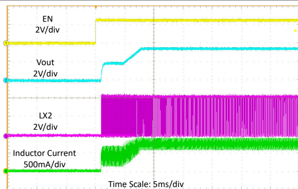
Figure 9-10. Switching Waveforms, Buck Operation with 1-A Load
