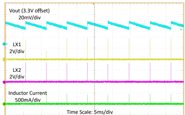
Figure 9-9. Switching Waveforms with 1-A Load
