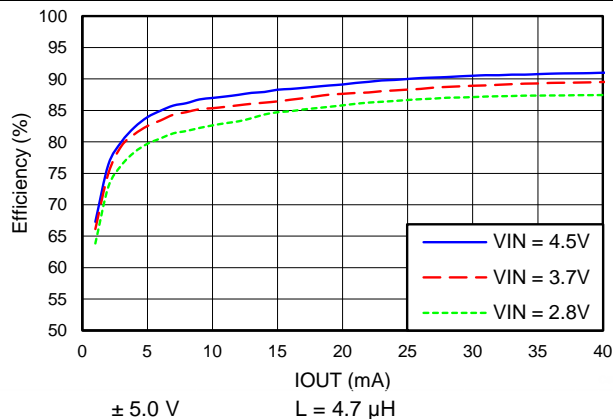
Figure 20. Combined Efficiency — 40mA Mode
