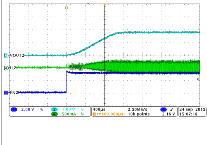
Figure 57. PWM Mode, Buck2, Soft-Start With No Load
