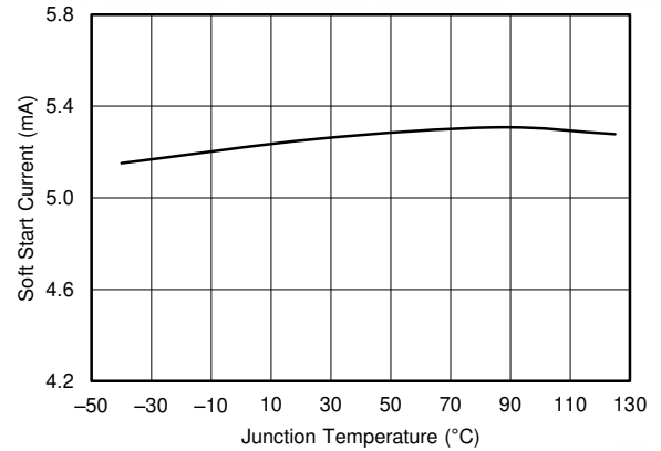
Figure 20. SS Pin Charge Current vs Temperature
