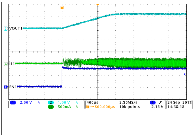
Figure 55. PWM Mode, Buck1, Soft-Start With No Load
