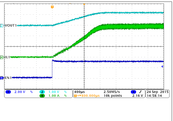
Figure 56. PWM Mode, Buck1, Soft-Start With Full Load
