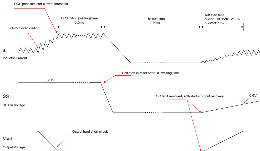
Figure 28. Overcurrent Protection
