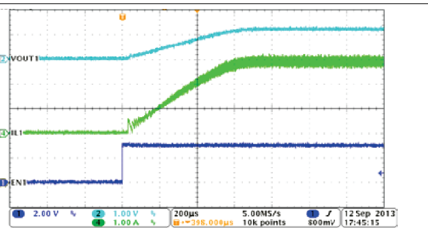
Figure 32. PSM Mode Buck1, Soft-Start With Full Load
