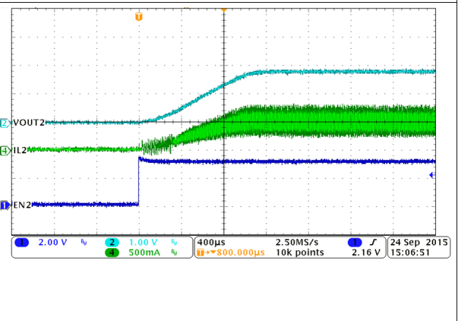
Figure 58. PWM Mode, Buck2, Soft-Start With Full Load
