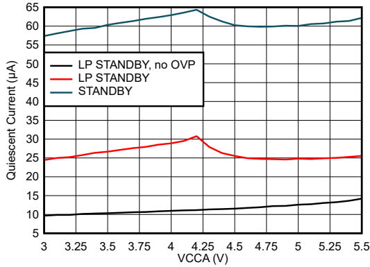
图 7-1. Quiescent Current vs Input Voltage
