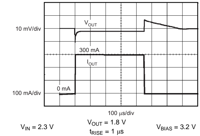
Figure 24. Load Transient Response
