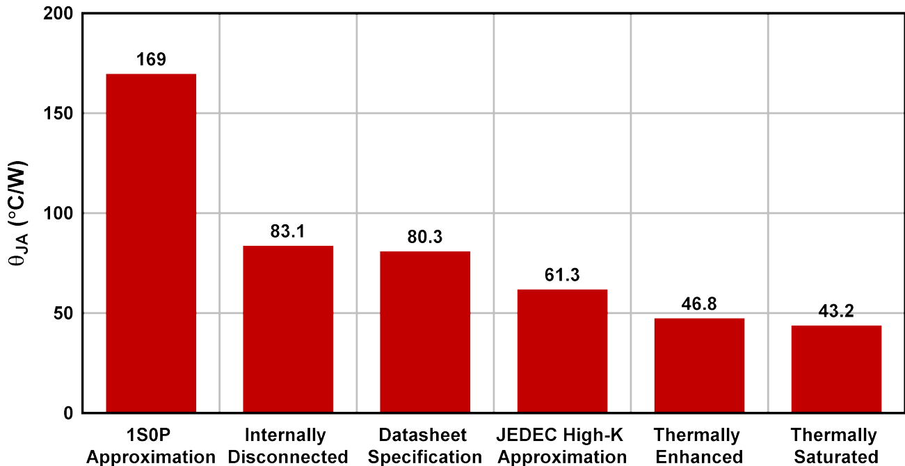
图 8-8. TPS746-Q1 (WSO) R_{\theta JA} vs Board Layout
