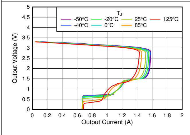
图 6-23. 3.3-V Foldback Current Limit vs I_{OUT}
