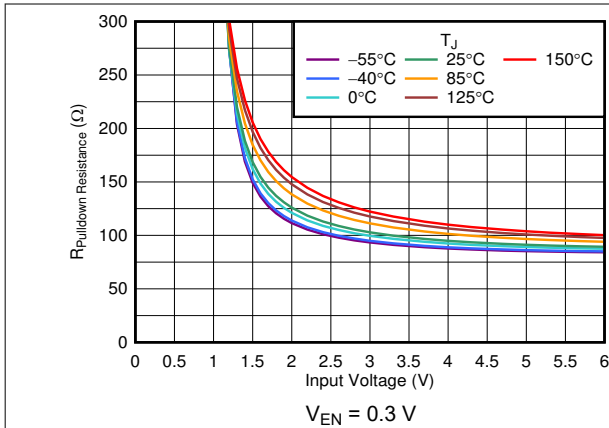
图 6-19. Pulldown Resistor ( R_{Pulldown} ) vs V_{IN}
