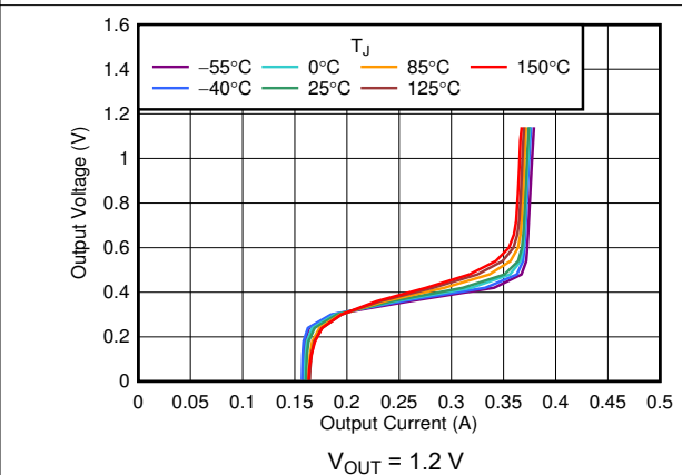
图 6-22. Foldback Current Limit vs I_{OUT} and Temperature
