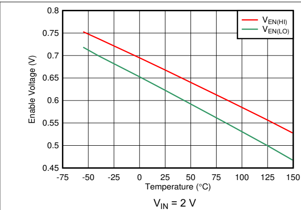
图 6-20. V_{EN(HI)} and V_{EN(LO)} Thresholds vs Temperature
