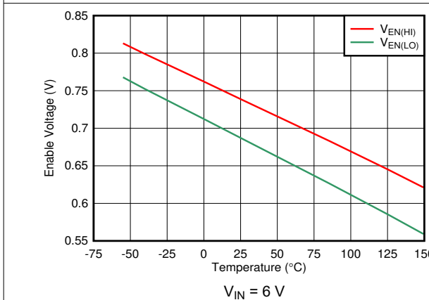
图 6-21. V_{EN(HI)} and V_{EN(LO)} Thresholds vs Temperature
