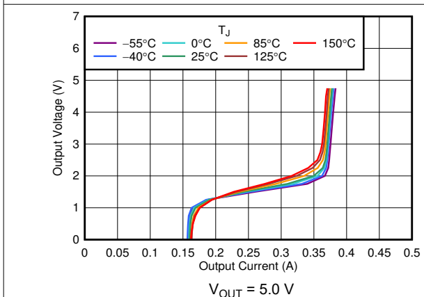
图 6-23. Foldback Current Limit vs I_{OUT} and Temperature
