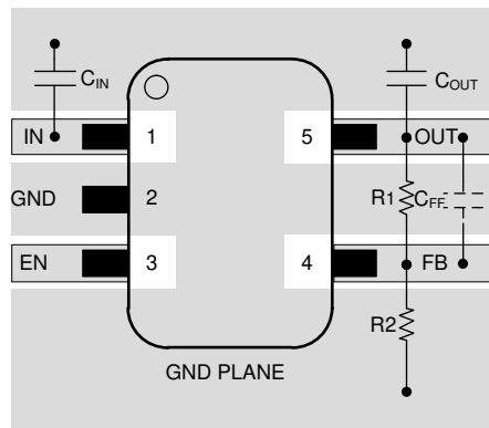
图 10-7. Layout Example for the DBV Package Adjustable Version
