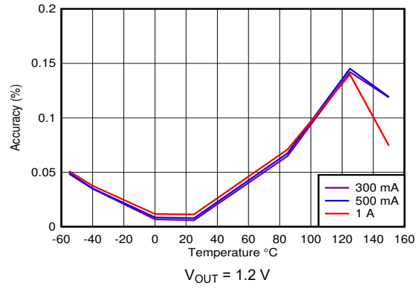
图 6-4. Output Accuracy vs Temperature
