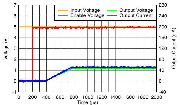
图 6-28. Start-Up Inrush Current With C_{OUT} = 1\text{ }\mu\text{F}
