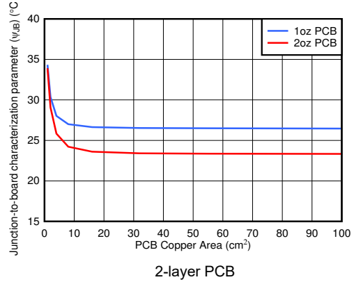
图 10-4. Junction-to-Board Characterization Parameter ( \psi_{JB} ) vs PCB Copper Area (DRB Package)
