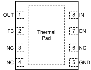
图 5-2. DRB Package (Adjustable), 8-Pin VSON (Top View)
